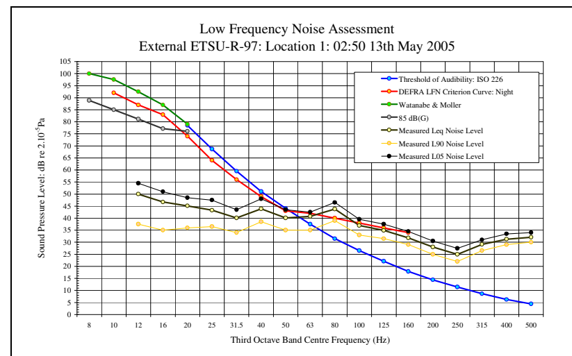
LFN Audibility External ETSU-R-97 13/05/05 Figure 19
