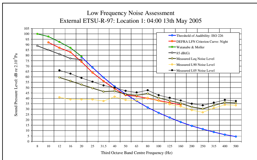
LFN Audibility External ETSU-R-97 13/05/05 Figure 25
