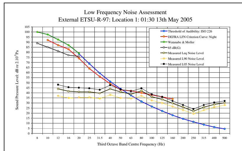
LFN Audibility External ETSU-R-97 13/05/05 Figure 11
