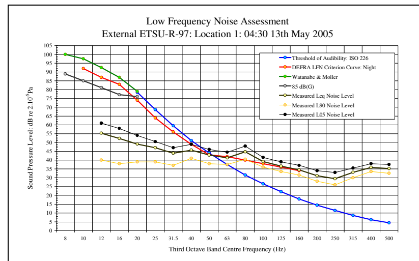
LFN Audibility External ETSU-R-97 13/05/05 Figure 27
