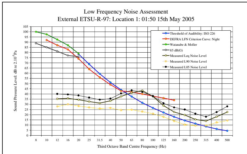
LFN Audibility External ETSU-R-97 15/05/05 Figure 10
