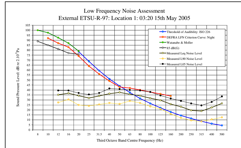
LFN Audibility External ETSU-R-97 15/05/05 Figure 19
