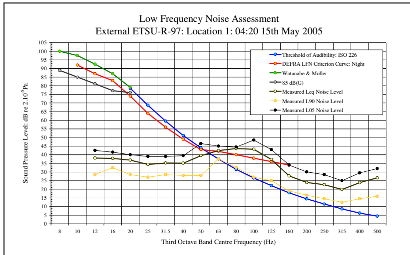
LFN Audibility External ETSU-R-97 15/05/05 Figure 25
