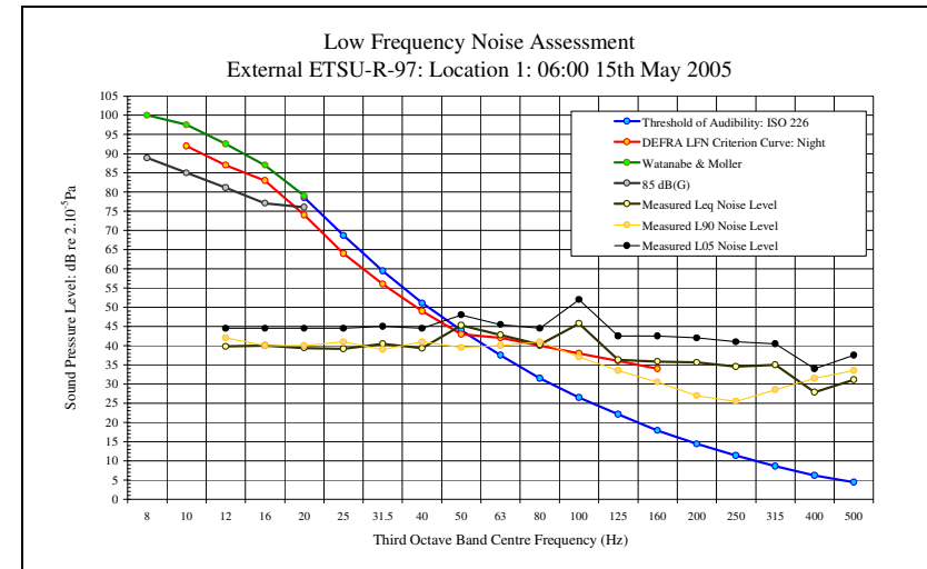
LFN Audibility External ETSU-R-97 15/05/05 Figure 35
