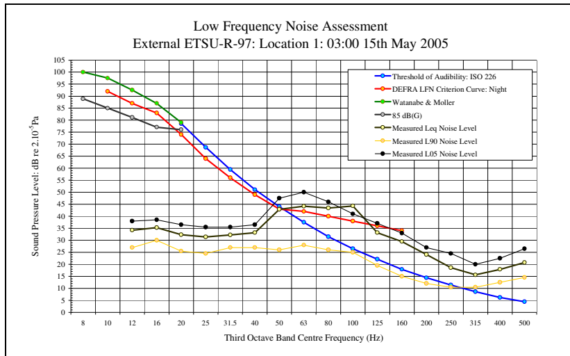
LFN Audibility External ETSU-R-97 15/05/05 Figure 17
