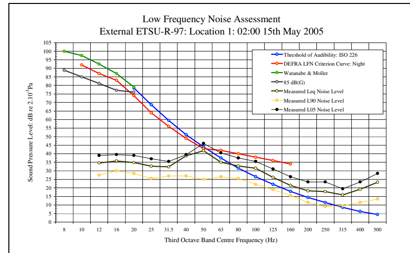
LFN Audibility External ETSU-R-97 15/05/05 Figure 11
