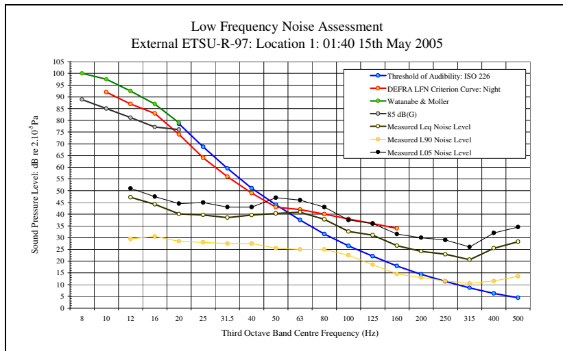
LFN Audibility External ETSU-R-97 15/05/05 Figure 9
