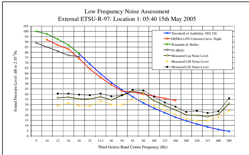
LFN Audibility External ETSU-R-97 15/05/05 Figure 33
