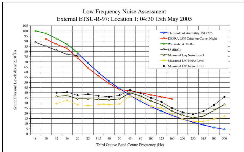
LFN Audibility External ETSU-R-97 15/05/05 Figure 26
