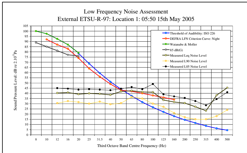
LFN Audibility External ETSU-R-97 15/05/05 Figure 34
