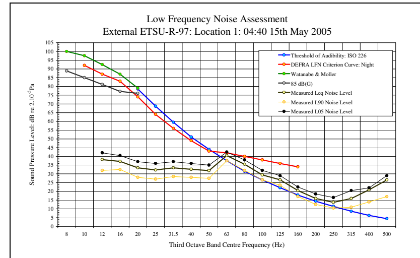
LFN Audibility External ETSU-R-97 15/05/05 Figure 27
