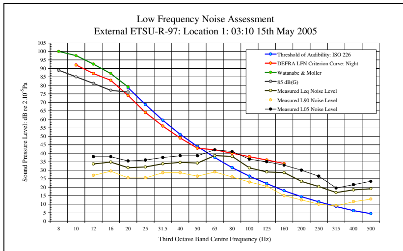
LFN Audibility External ETSU-R-97 15/05/05 Figure 18
